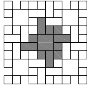
(L) 3 piece 7x7 - 33% 7x14 - 45% 14x14 - 22% Laying Ratio: 6:4:1
