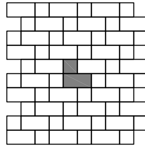
(C) 2 piece 7x7 - 34% 7x14 - 66% Laying Ratio: 1:1
