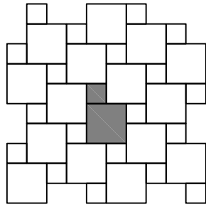
(B) 2 piece 7x7 - 20% 14x14 - 80% Laying Ratio: 1:1
