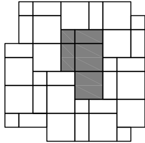
(J) 3 piece 7x7 - 8% 7x14 - 31% 14x14 - 61% Laying Ratio: 1:2:2
