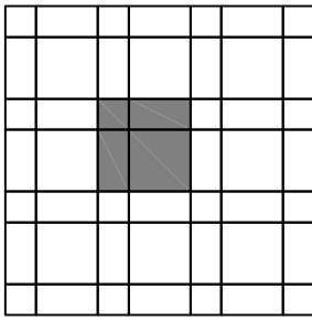
(A) 3 piece 7x7 - 10% 7x14 - 45% 14x14 - 45% Laying Ratio: 1:2:1
