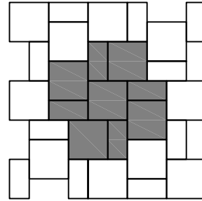
(K) 2 piece 7x14 - 29% 14x14 - 71% Laying Ratio: 4:5
