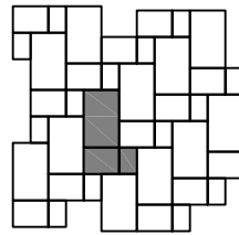
(I) 3 Piece 4x6 - 19% 6x8 - 23% 8x13 - 58% Laying Ratio: 1:1:1
