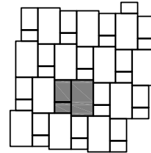
(K) 3 Piece 4x6 - 19% 6x8 - 23% 8x13 - 58% Laying Ratio: 1:1:1
