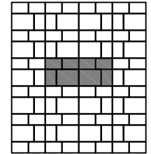
(L) 2 piece 4x6 - 60% 6x8 - 40% Laying Ratio: 6:2
