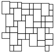
(G) 3 Piece Random 4x6 - 19% 6x8 - 23% 8x13 - 58% Laying Ratio: 1:1:1
