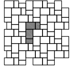
(F) 2 piece 4x6 - 34% 6x8 - 66% Laying Ratio: 2:2
