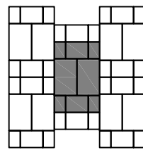
(J) 3 Piece 4x6 - 24% 6x8 - 24% 8x13 - 52% Laying Ratio: 4:2:2
